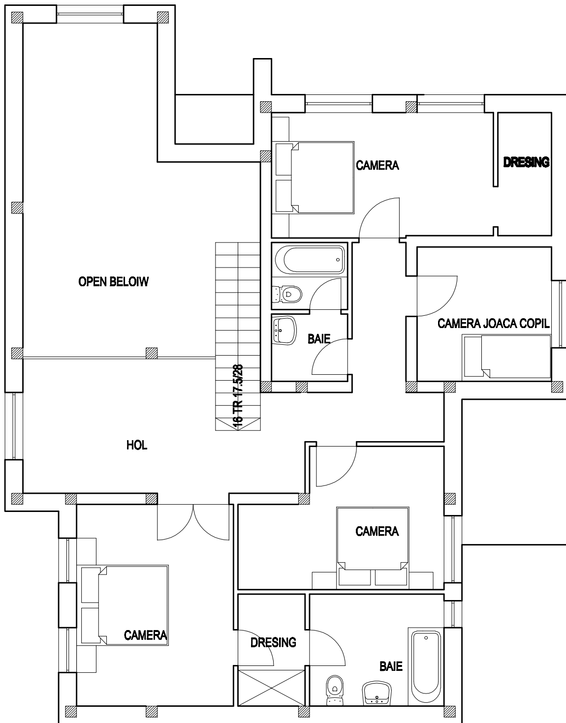
CASA PALMS PLAN MANSARDA
