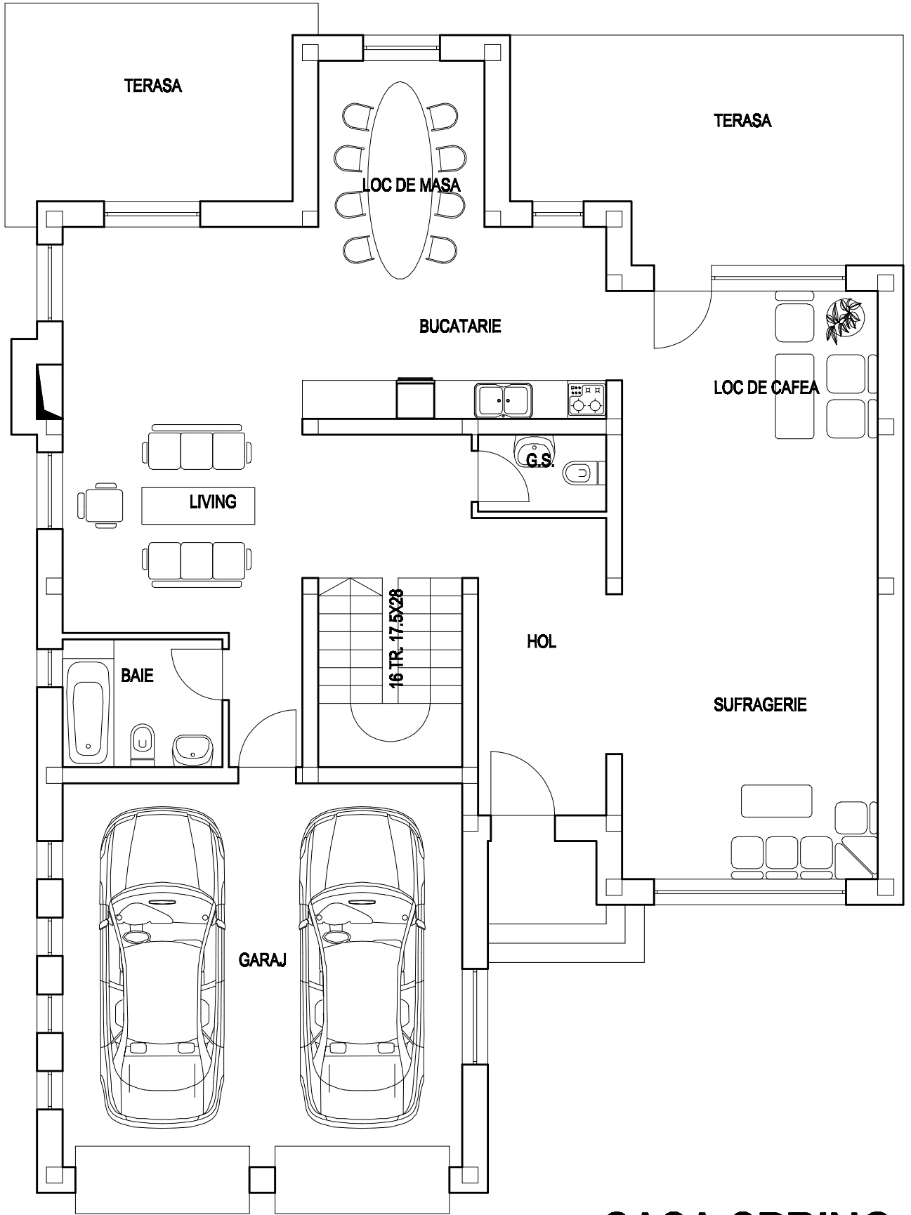
CASA SPRING PLAN PARTER
